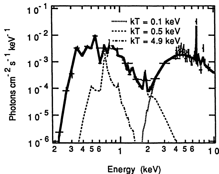
Fig. 2. \eta Car 0.2-10 keV spectrum from PSPC, IPC and BBXRT observations
