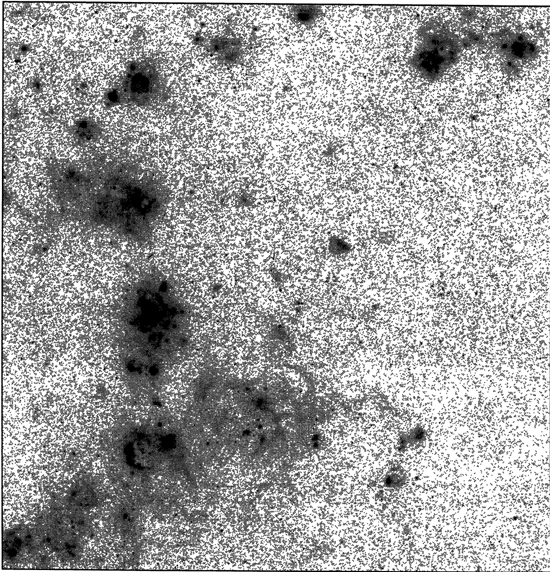
Fig. 2. Narrow band H\alpha WFC-2 image of M101 covering a field of about 2.7 \times 2.7 \text{ kpc}^2 in the lower right of the box in Figure 1.
