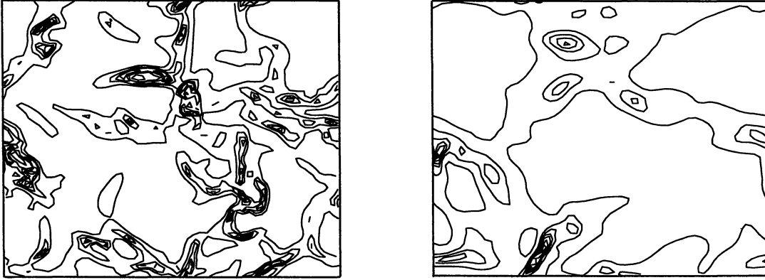
Fig. 2. Contour plots of the density field for the same run as in Fig. 1, a) (left) at t = 3.9 \times 10^7 and b) (right) at t = 15.1 \times 10^7 , showing the trend towards homogenization at late times, apparently induced by gravity.
