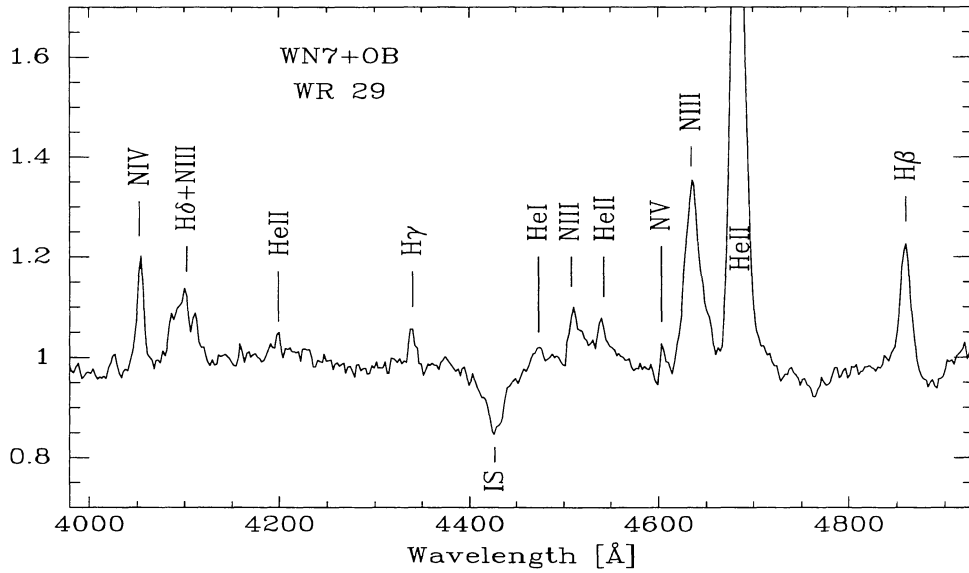
Fig. 1. Spectrum of WR29 obtained during the minimum radial velocity of the WN7 component. Note the faint absorption lines of the OB component to the red of the WN emissions with P Cyg profiles.
