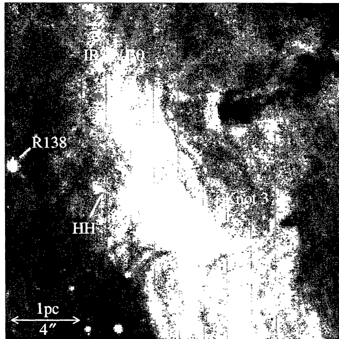
Fig. 5. Enlargement of WFC2/F656N ( H\alpha ) image of the W filament in the neighborhood of Knot 3. The jet-like structure resembling galactic Herbig-Haro objects is marked with “HH”. IRSW-30 (from Rubio et al. 1998), in the head of a bright-rimmed pillar, is one of the most luminous IR sources in the whole 30 Dor Nebula. R138 is an A supergiant field star not related to the young structures.
