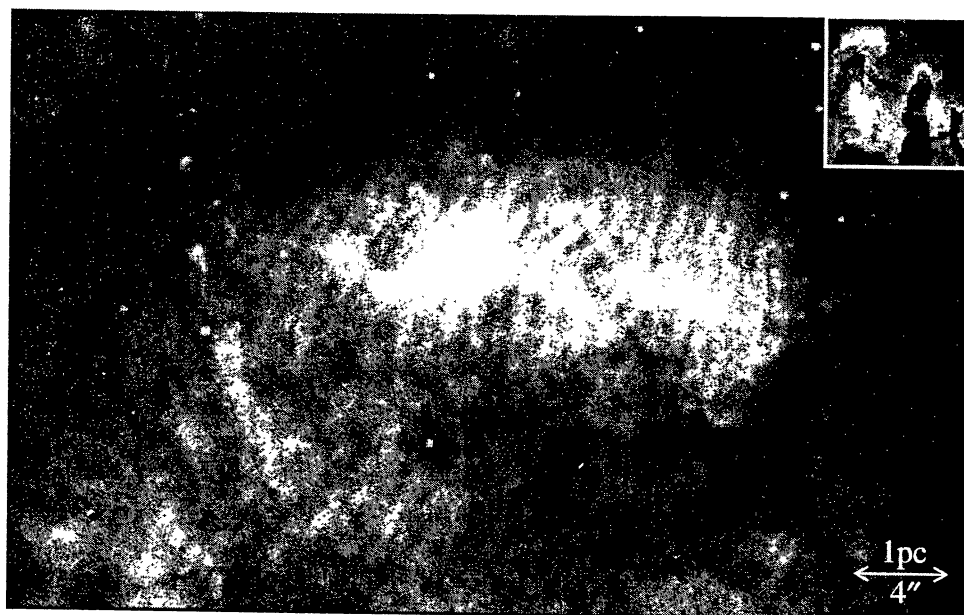
Fig. 3. WFC2/F656N ( H\alpha ) view of “30 Dor Southern Pillars”, a dusty structure 1' to the S of R136 that resembles the M16 Pillars. The inset in the upper right corner shows an M16 image (from Hester et al. 1996) scaled to the LMC distance.
