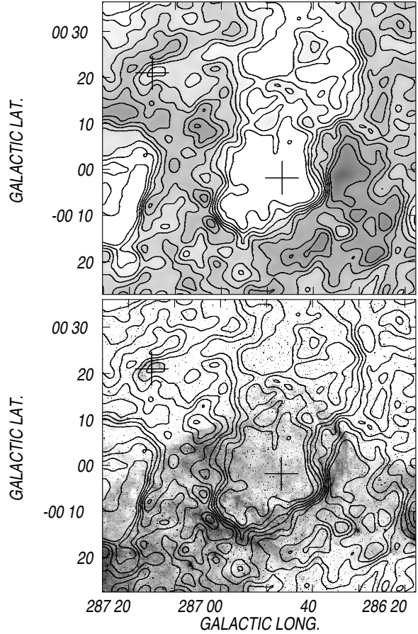
Fig. 2. Upper panel: HI column density distribution within the velocity interval -21.4 to -12.0 \text{ km s}^{-1} . The grayscale corresponds to 13.0 \times 10^{20} to 25.0 \times 10^{20} \text{ cm}^{-2} . The contour lines correspond to 12.4 \times 10^{20} to 18.0 \times 10^{20} \text{ cm}^{-2} in steps of 0.8 \times 10^{20} \text{ cm}^{-2} . As in Fig. 1, the crosses indicate the position of the massive stars. Lower panel: Overlay of the \text{H}\alpha (grayscale) and HI (contours) emission.
