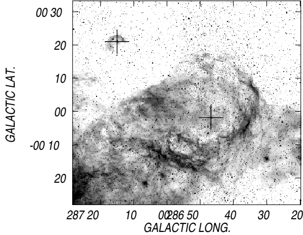
Fig. 1. DSS image showing the ring nebulae Anon(WR 23) around HD 92809, (l, b) = (286^{\circ}78, -0^{\circ}03) , and RCW 52 around LS 1887, (l, b) = (287^{\circ}25, +0^{\circ}35) . The crosses mark the position of the stars.
