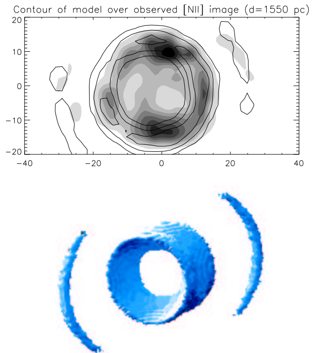
Fig. 1. Observed image compared with model image for d = 1550 pc and three-dimensional model structure used.
