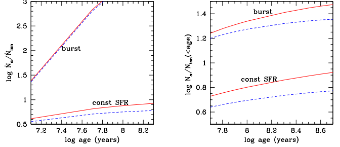
Fig. 4: Left : Continuum Ly \alpha photon emission rate \dot{N}_\alpha ( \text{s}^{-1} ) versus age (in years) for a stellar population with a Salpeter IMF ( dashed lines ) and a Scalo IMF ( solid lines ). Upper curves assume an instantaneous burst of star formation, lower curves a constant star formation rate. The rate of production of Ly \alpha photons has been normalized to the rate of emission of hydrogen-ionizing photons, \dot{N}_{\text{ion}} . The population synthesis values have been computed for low metallicities ( Z = 0.02 Z_\odot ), and are based on an update of Bruzual & Charlot’s (1993) libraries. Right : Same after integration over the age of the stellar population.
