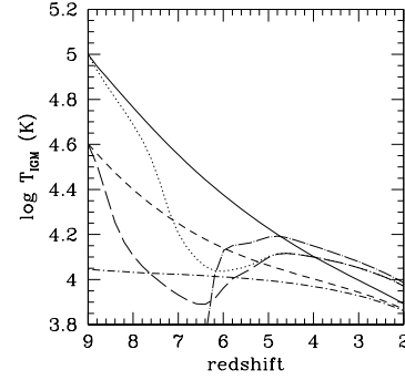
Fig. 1: Thermal history of intergalactic gas at the mean density in an Einstein–de Sitter universe with \Omega_b h^2 = 0.02 and h = 0.5 . Short dash-dotted line : temperature evolution when the only heating source is a constant ultraviolet (CUV) background of intensity 10^{-22} \text{ ergs cm}^{-2} \text{ s}^{-1} \text{ Hz}^{-1} \text{ sr}^{-1} at 1 Ryd and power-law spectrum with energy slope \alpha = 1 . Long dash-dotted line : same for the time-dependent quasar ionizing background as computed by Haardt & Madau (1996; HM). Short-dashed line : heating due to a CUV background but with an initial temperature of 4 \times 10^4 K at z = 9 as expected from an early era of pregalactic outflows. Long-dashed line : same but for a HM background. Solid line : heating due to a CUV background but with an initial temperature of 10^5 K at z = 9 . Dotted line : same but for a HM background.
