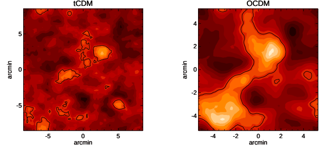
Fig. 3: Left: Radio map of redshifted 21-cm emission against the CMB in a ‘tilted’ CDM (tCDM) cosmology at z = 8.5 . Here a collisionless N -body simulation with 64^3 particles has been performed with Hydra (Couchman et al.1995). The simulation box size is 20h^{-1} comoving Mpc, corresponding to 17 (11) arcmin in tCDM (OCDM). The baryons are assumed to trace the dark matter distribution without any biasing, the spin temperature to be much greater than the temperature of the CMB everywhere, and the gas to be fully neutral. The point spread function of the synthesized telescope beam is a spherical top-hat with a width of 2 arcmin. The frequency window is 1 MHz around a central frequency of 150 MHz. The contour levels outline regions with signal greater than 4\mu\text{Jy} per beam. Right: Same for an open cosmology (OCDM). Since the growth of density fluctuations ceases early on in an open universe (and the power spectrum is normalized to the abundance of clusters today), the signal at a given angular size is much larger in OCDM than in tCDM at these early epochs. (From Tozzi et al.2000.)
