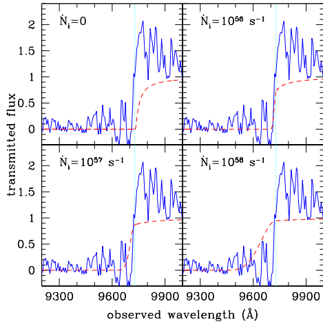
Fig. 6: The Keck/LRIS spectrum of the faint z_{\text{em}} = 5.5 quasar RD J0301117+002025 (Stern et al. 2000), redshifted to z_{\text{em}} = 7 . The dotted vertical lines indicate the expected wavelength of the Ly \alpha resonance. Fluxes have arbitrary normalizations. The dashed curves show the transmission \exp(-\tau_{\text{GP}}) (where \tau_{\text{GP}} is the Gunn-Peterson optical depth to resonant scattering) through a uniform IGM, assuming the QSO is being observed prior to the reionization epoch at z_r = 6 . Four different cases are shown, as the rate of emission of Lyman continuum photons which ionize the IGM in the vicinity of the source is varied from \dot{N}_i = 0 to \dot{N}_i = 10^{56}, 10^{57} , and 10^{58} \text{ s}^{-1} . The calculations assume a quasar lifetime of t_s = 10^7 \text{ yr} , a power-law spectrum of the form f_\nu \propto \nu^{-\alpha} with \alpha = 0.5 near the hydrogen Lyman edge, a recombination timescale of t_{\text{rec}} = 1.3 \text{ Gyr} , an Einstein-de Sitter universe with h = 0.5 , and a baryon density parameter \Omega_B h^2 = 0.02 . (From Madau & Rees 2000.)
