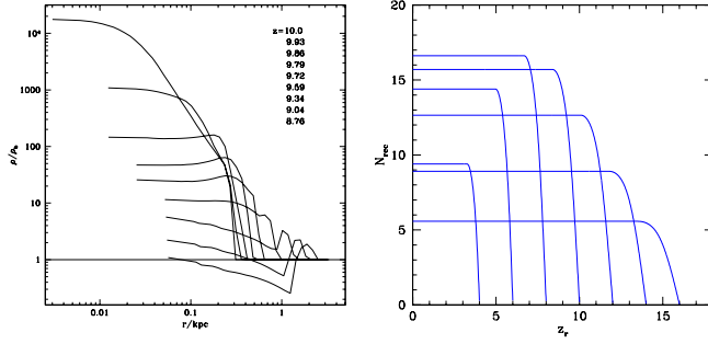
Fig. 5: Left : The evolution of the density profile of a minihalo with mass 10^6 M_\odot , illuminated by a UV background flux at z = 10 . The hydrogen photoionization rate is assumed to be uniform on the grid, i.e. we do not solve radiative transfer. Photoevaporation occurs very rapidly, with most recombinations occurring within a sound-crossing time. The figure reveals that by z = 9.5 the density contrast is everywhere reduced below \delta \lesssim 10 . Right : Total number of recombinations inside minihalos, following sudden reionization at redshift z_r . Recombinations are shown per background hydrogen atom. In the earliest stages of reionization, minihalos dominate the average gas clumping in the universe, and can therefore dominate the total recombination rate. (From Haiman et al.2001.)
