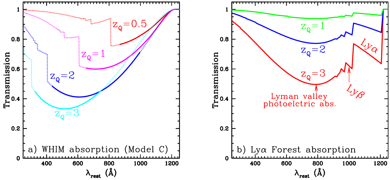
Fig. 2. Rest-frame transmission curves for quasars of representative redshifts. (a) using an H I absorption density corresponding to Model C. (b) using a distribution of Ly \alpha forest absorbers similar to Zheng et al. (1997). The large discontinuity in each curve in Panel a always occurs in the observer-frame at 1216 Å.
