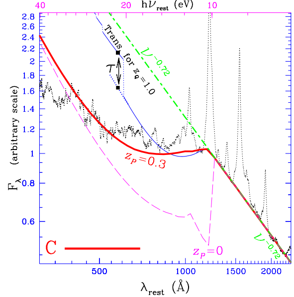
Fig. 1. The dotted-line in this F_\lambda vs \lambda_{rest} plot represents the composite spectrum of radio-quiet quasars by TZ02. The straight short-long dashed line represents a power-law fit (of index -0.72 ), in the longer wavelength region \lambda > 1200 \text{ \AA} ( \lambda_{rest} ) of the continuum underlying the emission lines. The thick solid line overlaying the TZ02 data is our synthetic composite Model C, which assumes a single intrinsic power-law, F_\nu \propto \nu^{-0.72} and a tenuous H I absorption screen described by eq. (1) with n_{H^0}^0 = 5.2 \times 10^{-12} \text{ cm}^{-2} and z_P = 0.3 . The staircase thin continuous line represents the transmitted spectrum for an individual quasar of redshift z_Q = 1.0 , assuming eq. (1) [same Model C] and an ideal detector with sensitivity at all wavelengths. The natural logarithm of the flux jump between the two filled squares is \tau_{1160} (see definition in §6). The thin long-dashed line illustrates the discontinuity at \lambda_{rest} = 1216 \text{ \AA} if we set z_P to zero in Model C (i.e. without cavity).
