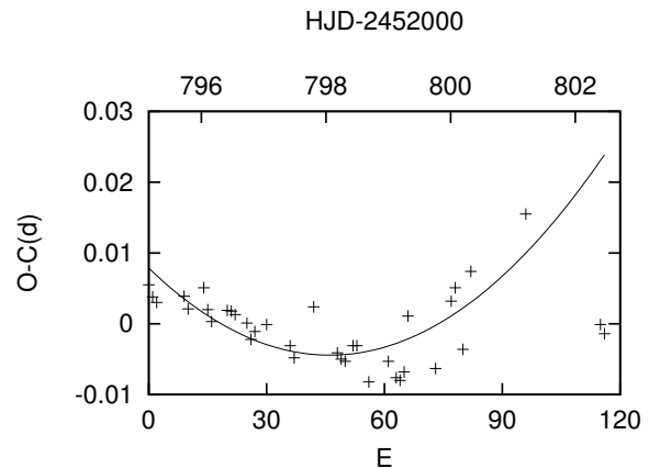
Fig. 2. O-C diagram of superhump maxima. The abscissa denotes the cycle count since 2452795.1515.
