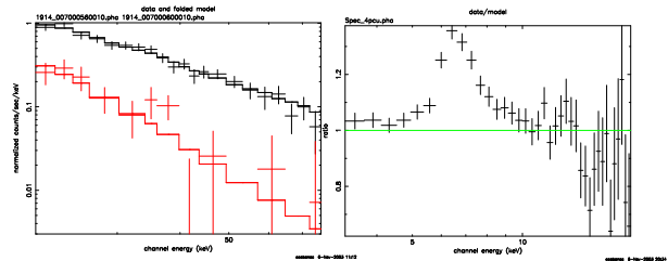
Fig. 1. Left 20-80 keV ISGRI spectra of the source during rev#70 separated by 8.6 ks. Resulting photon index are 2.210.15 (black) and 3.81.0 (red). Right Ratio between the RXTE-PCA data and the model chosen (simple power-law with N_H fixed to 5.6 \cdot 10^{22} \text{ cm}^{-2} ).
