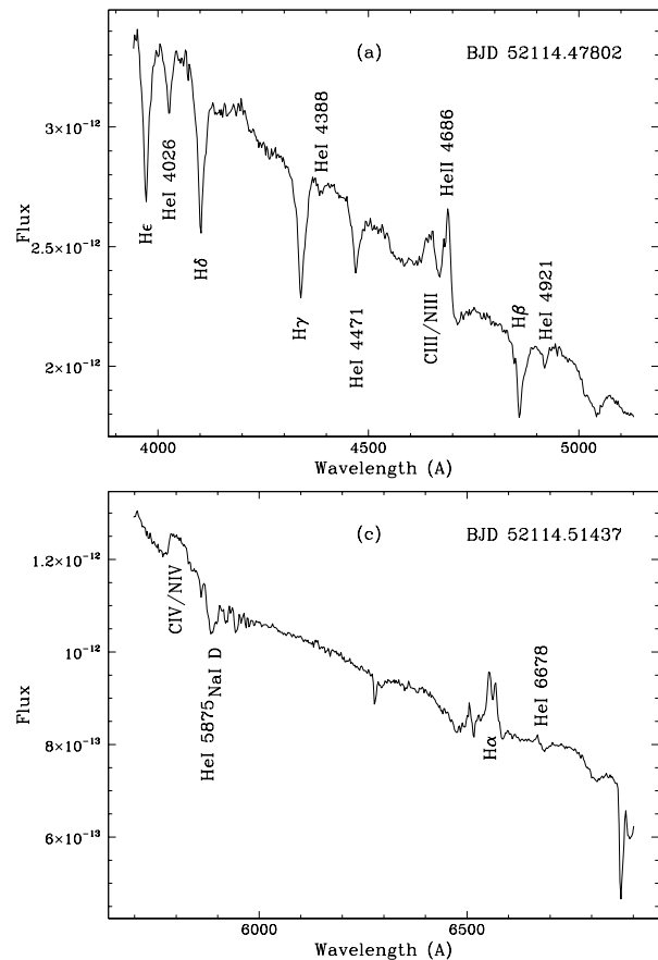
Fig. 1. Spectra around the outburst maximum. We can see emission lines of H\alpha , He II 4686, C III/N III around 4630, and C IV/N IV around 5800, and absorption lines of other Balmer lines, He I, and Na I D on a blue continuum.
