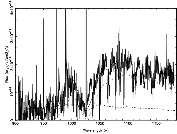
Fig. 2. The best-fitting composite white dwarf plus hot accretion belt model to the FUSE spectrum of SS Aur. The white dwarf flux is the dotted line, the accretion belt flux is the dashed line and the sum of the two is the solid line.
