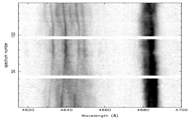
Fig. 1. Trailed spectrogram of the Bowen blend and He II \lambda 4686 line showing the Doppler shift of the narrow C III and N III components. From Steeghs & Casares (2002).
