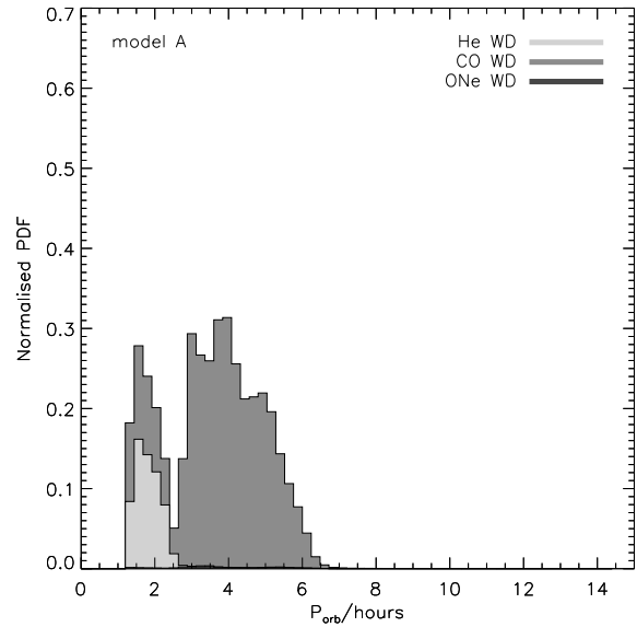
Fig. 3. Predicted orbital period distributions of CVs that evolve under the influence of a circumbinary disc.
