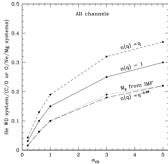
Fig. 1. Ratio of He white dwarf - MS star binaries to C/O or O/Ne WD-MS star binaries for different initial mass ratio or initial secondary mass distributions, as a function of the common-envelope ejection efficiency \alpha_{CE} for WD-MS binaries forming through all considered formation channels.
