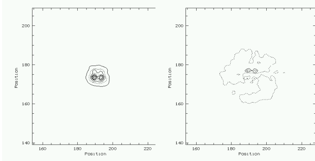
Fig. 1. Contour plot of the original (left) and residual (right) intensity distributions for HIP 25550
