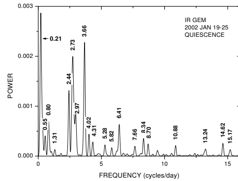
Fig. 3. CLEAN spectrum of the complete set of the de-trended time series, showing a strong signal at 0.21 c/d . The complicated pattern suggests multi-periods. Spikes at 14.62 and 15.17 c/d can also be seen.
