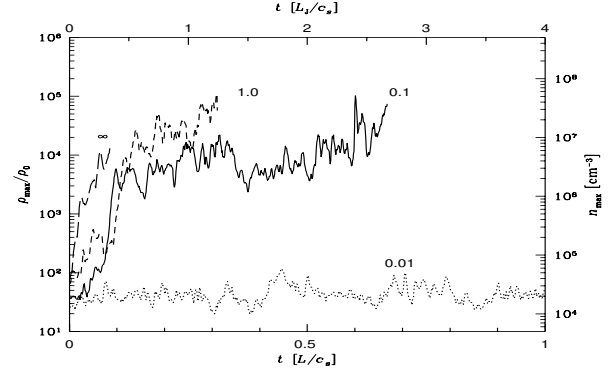
Fig. 1. Evolution of the global maximum of the density field for all runs considered here. The numbers indicate the corresponding values of \beta .
