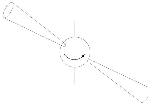
Fig. 2. The phenomenological “hollow cone model”, where “beams” are emitted from the magnetic polar caps. Although not in the least an aligned model, it is often mistaken as supporting the aligned MHD model in Figure 1
