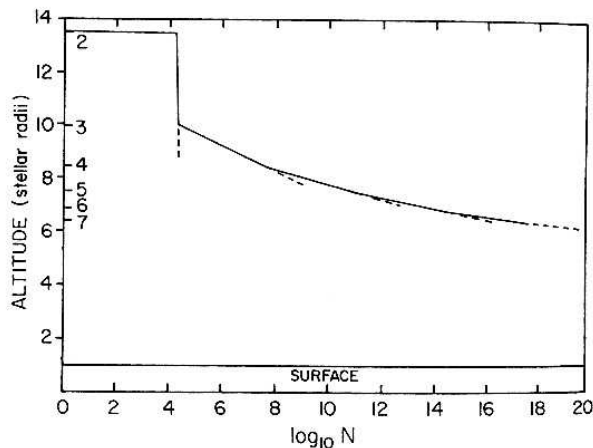
Fig. 8. Exponential growth of a bunch by pair production. The process has been assumed to happen all at once every gamma-ray mean-free-path, which produces the sharp steps. The process also works for “millisecond” pulsars because the much smaller magnetic fields are compensated by the proportionately larger spin rates.
