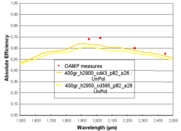
Fig. 5. Measured and computed transmission of the ruled grating in the K band. The lines represent the calculated transmission, for TE and TM unpolarized light, and the solid dots, actual measurements in the demonstration sample.
