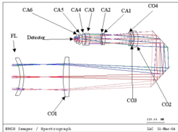
Fig. 3. Optical layout as disposed in the instrument.
