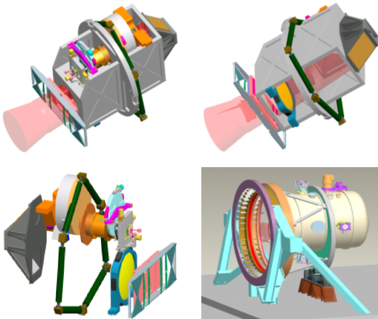
Fig. 6. Different views of the EMIR cold bench. Top left: upper view showing the CSU, periscope, second collimator barrel, grism wheel, camera barrel, filter wheels and the detector mount table. Top right: view from the bottom on which the CSU, first collimator barrel and the periscope are seeing. Bottom left: schematic of the different subsystems positioned along the incoming beam, without the cold bench. The support trusses are also shown. Bottom right: the EMIR cryostat attached to the Nasmyth rotator.
