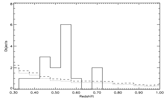
Fig. 4. The figure shows as a function of redshift: ( dotted ) the mean number of objects in a region of 2 \times 2 arcmin 2 of the Deep Lens Survey field shown in Fig. 2. ( Dashed ) the expected 1\sigma upper limit for a random Poisson distribution, and ( solid ) the actual distribution of objects in such region. A clear overdensity exists at z \sim 0.6 .
