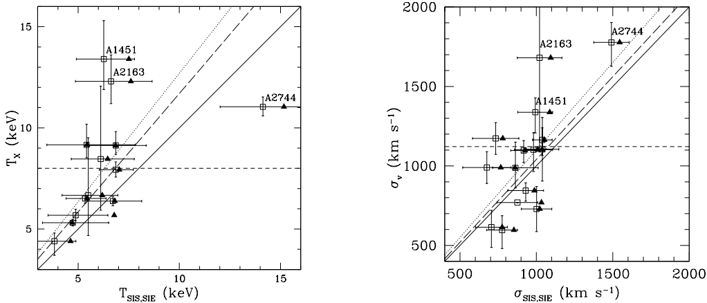
Fig. 1. Comparison between the actually measured ICM temperatures (left panel) and velocity dispersions (right panel) with those inferred by the fitting of isothermal profiles (spheric-SIS and elliptical-SIE) to the shear data. The squares correspond to the spherical model and triangles to the elliptical. The error bars of the latter were suppressed for clarity. The solid line is defined by T_{SIS,SIE} = T_X or \sigma_{SIS,SIE} = \sigma_v . The dotted and long dashed lines show the best-fit obtained with the SIS and SIE models, respectively, when the origin is kept constant. The short dashed line indicates T_X = 8 keV. Clusters with higher temperatures show signals of dynamic activity.
