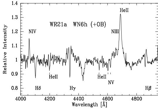
Fig. 1. Continuum rectified blue optical spectrum of WR 21a obtained at CASLEO.
