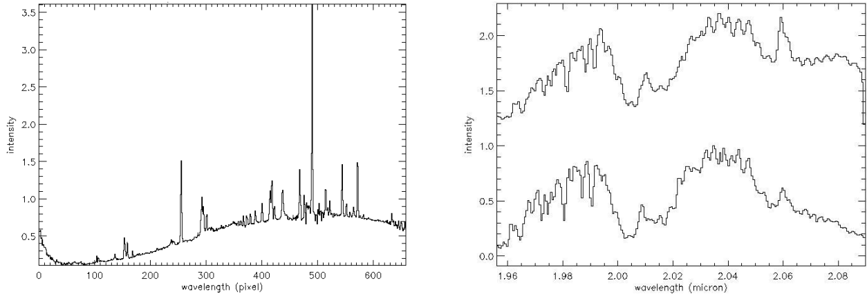
Fig. 1. Left Panel: A near-IR spectrum of IGR J16318–4848 obtained with the CorMASS spectrograph aboard the Magellan telescope. The spectral coverage is 0.8–2.4 \mu\text{m} (from the left to right) and resolution is \sim 300 . Right Panel: Sample spectra of two highly-obscured X-ray binaries around 2 \mu\text{m} obtained with the long-slit near-IR spectrograph of the Palomar Hale 5-m telescope. The spectral resolution is \sim 700 .
