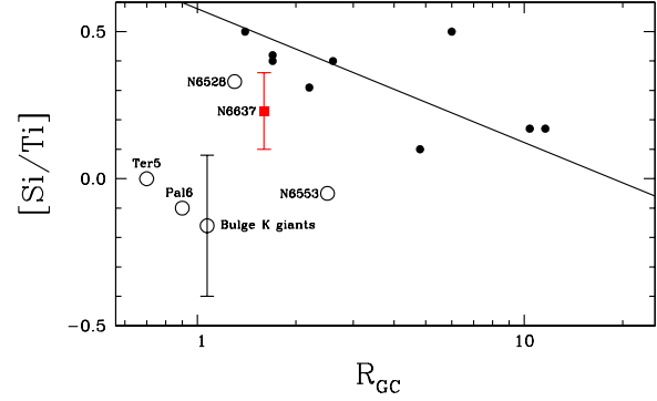
Fig. 4. [\text{Si}/\text{Ti}] as a function of R_{GC} . Dots represent 9 OHGCs analyzed by Lee (2007, in preparation). The solid line represents the bisector linear fit to the data. A non-parametric Spearman rank-order test indicates a probability of \approx 0.09\% that the anti-correlation between [\text{Si}/\text{Ti}] and R_{GC} of the clusters is random.
