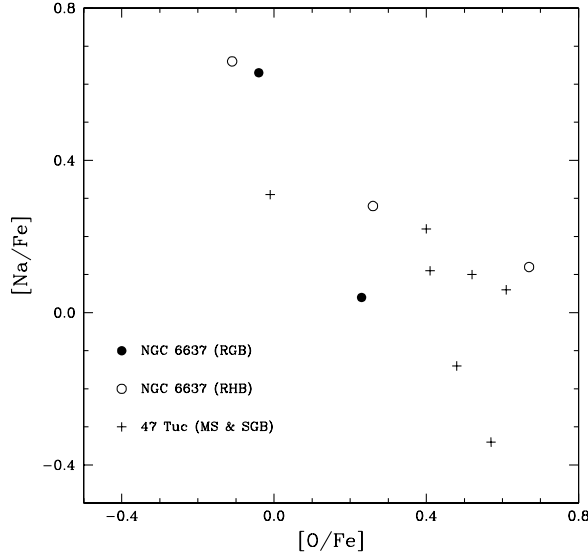
Fig. 2. A comparison of [\text{Na}/\text{Fe}] vs. [\text{O}/\text{Fe}] for MS and SGB stars in 47 Tuc vs. RGB and RHB stars in NGC 6637.
