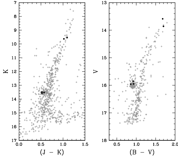
Fig. 1. Color-magnitude diagram of NGC 6637 showing the positions of our program stars.
