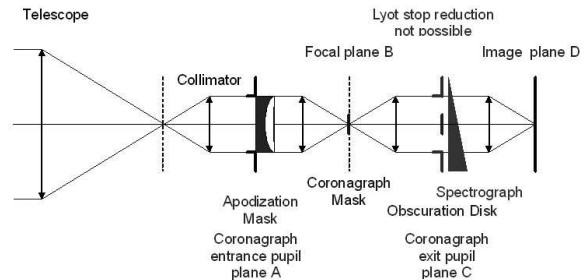
Fig. 1. Configuration for FRIDA optical assembly.
