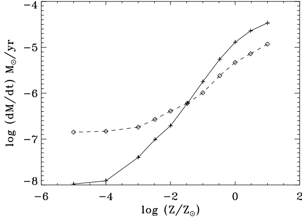
Fig. 1. Mass loss versus initial Z for late-type nitrogen-rich (WN) stars (solid line) and carbon-rich WC stars (dashed line). Note that metal self-enrichment is accounted for, but does not enter in our expression of Z . See Vink & de Koter (2005) for details.
