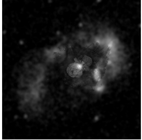
Fig. 2. Comparison of a CHANDRA X-ray image of \eta Carinae and an HST/WFPC2 image of the Homunculus. The X-ray emission is extended and associated with the "Outer Debris Field" which surrounds the bipolar Homunculus nebula. \eta Carinae is the optical- and X-ray-bright point at the center of the image. WFPC2 image courtesy of N. Smith and J. Morse.
