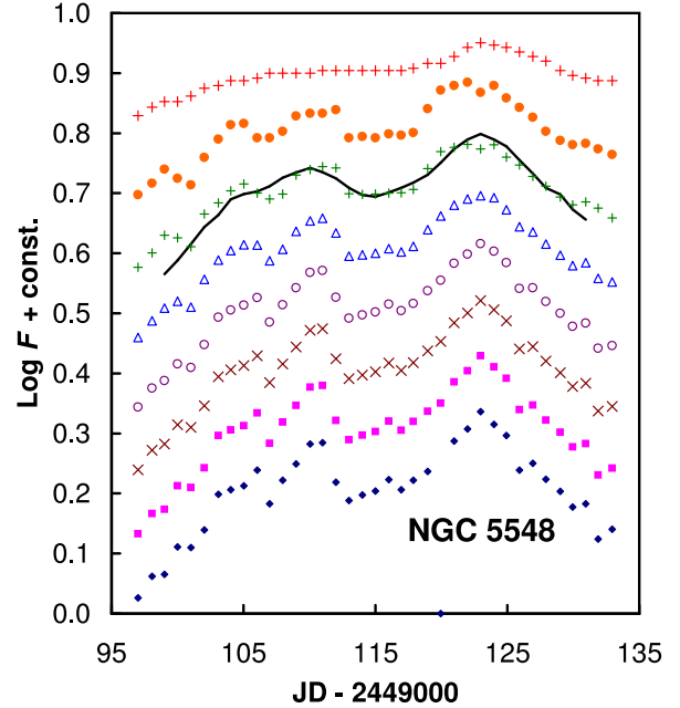
Fig. 5. Light curves for NGC 5548. Data from Korista et al. (1995). The light curves, starting from the bottom are, at \lambda\lambda 912 (extrapolated), 1145, 1350, 1460, 1790, 2030, 2195, and 5100. Notice the decreasing amplitudes and greater smoothness of the light curves as one goes to longer wavelengths. The smooth curve through the \lambda 2030 curve is the \lambda 912 light curve smoothed with a boxcar function running from -3 to +3 days.
