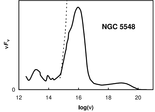
Fig. 2. The spectral energy distribution of NGC 5548 (solid line) and the spectrum of a F_\nu \propto \nu^{+1/3} accretion disk (dotted line). Compare this representation of the observed SED with Figure 1 above. (SED from Gaskell, Klimek, & Nazarova 2007).
