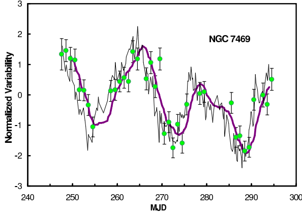
Fig. 6. The relative UV, \lambda 1315 , variability of NGC 7469 (thin line) compared with the optical, \lambda 4845 , variability (circles with error bars). The thick solid curve is the UV variability smoothed with a boxcar function extending from 0 to 5 days. The variations are shown on a linear scale normalized to the same variance (data from Wanders et al. 1997; Collier et al. 1998; Kriss et al. 2000).
