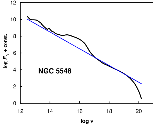
Fig. 1. The spectral energy distribution of NGC 5548 (thick curve) and a \nu^{-1} power law (thin line). Compare this representation of the data with Figure 2 below. (Data from Gaskell, Klimek, & Nazarova 2007).
