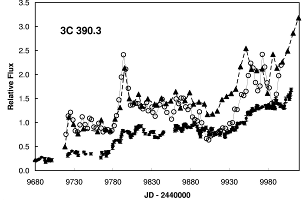
Fig. 7. Soft X-ray, UV, and optical fluxes of 3C 390.3. The open circles are 0.1–2 keV ROSAT HRI fluxes; the black triangles are IUE \lambda 1370 UV fluxes, and the small black circles with error bars are V-band fluxes. The ROSAT fluxes are from Leighly et al. (1997), the UV fluxes are based on O'Brien et al. (1998), and V-band fluxes have been derived with scalings and corrections from Dietrich et al. (1998). Scale factors have been chosen for plotting convenience, and an arbitrary constant has been subtracted from the V-band fluxes. Figure reproduced from Gaskell (2006).
