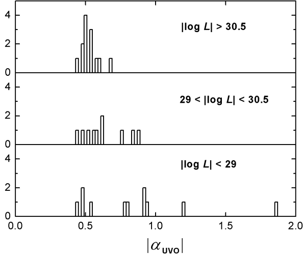
Fig. 3. The distribution of optical to UV spectral indices in AGN. Note that this figure, taken from Gaskell et al. (2004), uses the opposite sign convention for \alpha from this paper.
