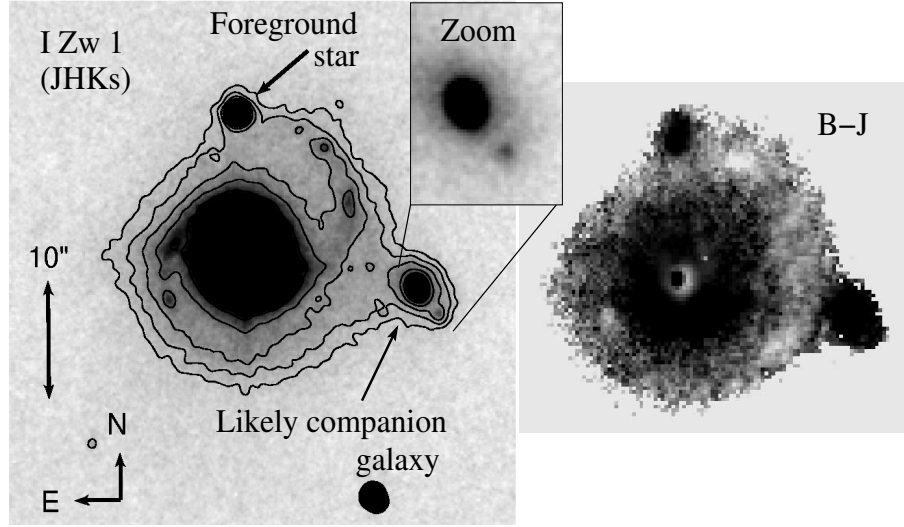
Fig. 1. Left panel: NIR image of I Zw 1 taken with ISAAC. The figure shows the average of the J -, H -, and K_s -band images. A zoom of the region around the likely companion highlights the separate object to the south-west of the companion. Right panel: B - J image of I Zw 1 with light and dark grey indicating blue and red colors, respectively. The central part of the color image shows artifacts from saturation by the QSO nucleus.
