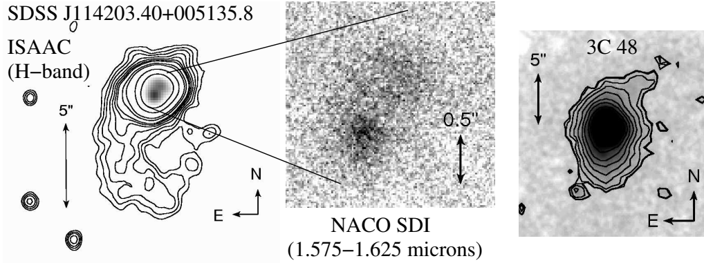
Fig. 2. Left panel: H -band ISAAC image of SDSS J114203.40+005135.8. The contours of the ISAAC image show the disturbed morphology of the QSO with the prominent extension to the south-west. The cuts of the underlying grey-scale image are adjusted to highlight the double structure in the center of the host galaxy. Middle panel: NACO SDI image of the central region. The plot shows a median of the four images taken simultaneously by the SDI at 1.575, 1.600, and 1.625 micron. Right panel: Averaged ISAAC J - and H -band image of the QSO 3C 48 for comparison (data published in Zuther et al. 2004).
