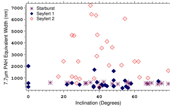
Fig. 2. Relation between the 7.7 \mu\text{m} PAH emission with the inclination angle.
