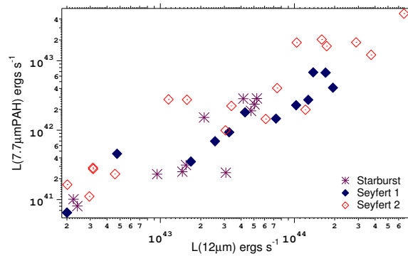
Fig. 1. Relation between the IRAS 12 \mu\text{m} luminosity and the 7.7 \mu\text{m} PAH emission.
