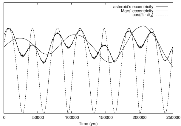
Fig. 3. The secular evolution of a particular asteroid.
