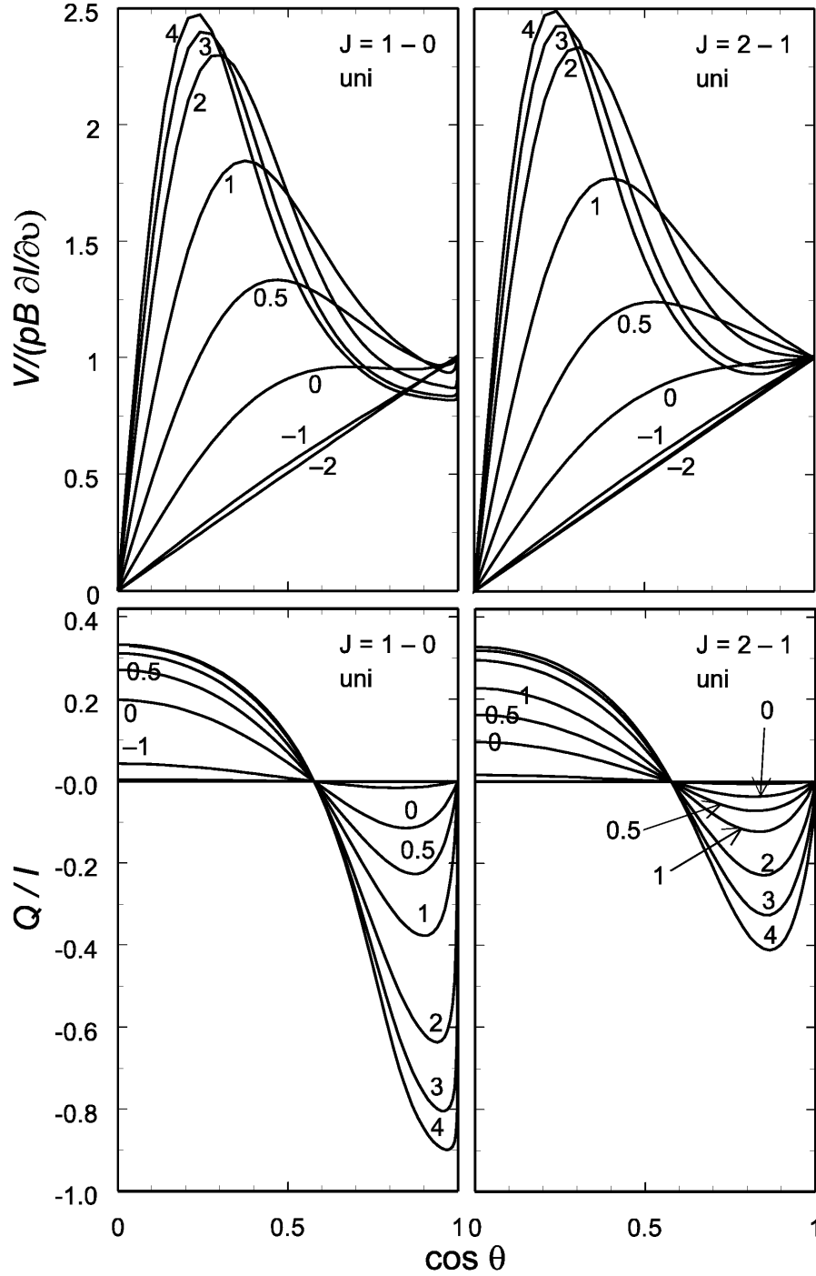
Fig. 1. Circular and linear polarization of maser radiation as a function of the cosine of the angle \theta between the direction of the magnetic field and the line of sight. Polarizations are presented for angular momentum J = 1 - 0 and J = 2 - 1 masers, in separate panels as indicated by the label in each panel. The curves are labeled by the \log_{10} of the saturation degree (upper panels). The circular polarization is measured by the magnitude of V/(pB \partial I/\partial \nu) which is equal to \cos \theta in the unsaturated limit (bottom panels). The fractional linear polarization, Stokes- Q is positive when the linear polarization is perpendicular to the direction of the magnetic field projected onto the plane of the sky (from Watson & Wyld 2001).
