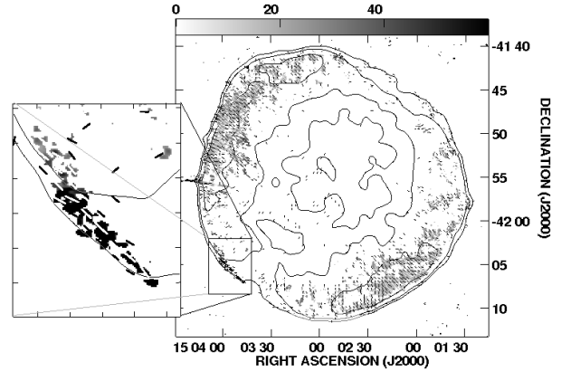
Fig. 1. Fractional polarization (greyscale) of SN 1006 with magnetic field vectors overlaid. The percentage fractional polarization is indicated at the top. The inset on the left shows an enlargement of the SE region, where the high polarization as well as the tangential direction of the magnetic field are evident. Radio continuum contours are included.
