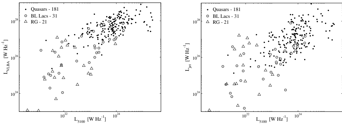
Fig. 1. The total radio luminosity of the VLBA jet at 15 GHz against optical continuum luminosity at 5100 Å, (left panel), and radio luminosity of the jet (unresolved core subtracted) against optical continuum luminosity at 5100 Å (right panel) for quasars, BL Lacs and radio galaxies.
