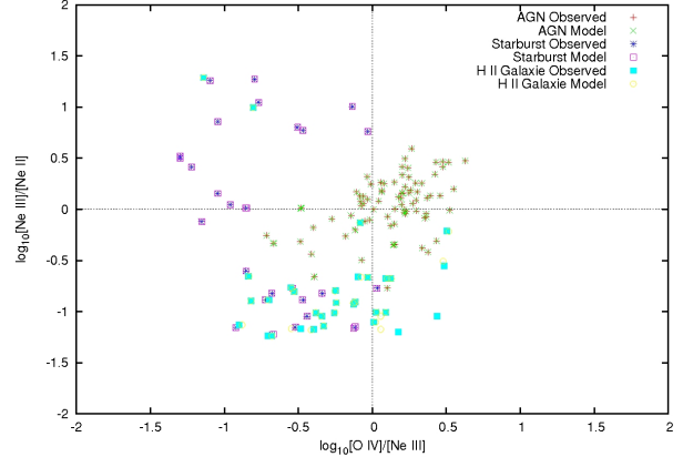
Fig. 1. Comparison between the [Ne III]/[Ne II] versus [O IV]/[Ne III] for a sample of BAT AGN, LINERs, starburst galaxies, HII galaxies and BCDs from (Weaver et al. 2010) and our two-zone models. The dashed lines represent a value of unity for the [Ne III]/[Ne II] and [O IV]/[Ne III] ratios.
