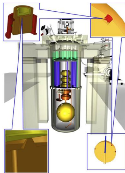
Fig. 2. A schematic view of the detector. The explosive view explains the principle of the two mode resonant transducer coupled to the spherical antenna.
