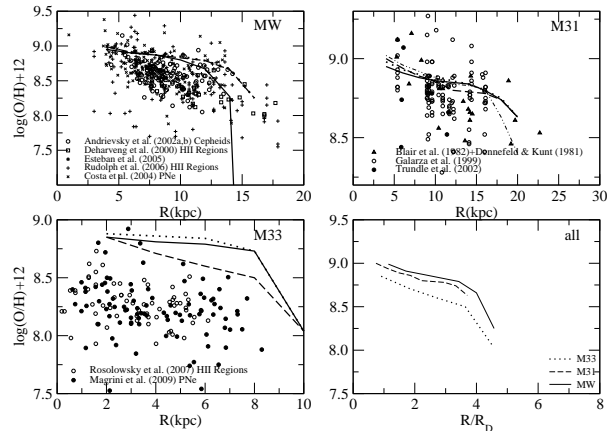
Fig. 1. Radial oxygen abundance gradient for the three galaxies in the sample. In these figures, different lines represent model outputs. See Marcon-Uchida et al. (2010) for the symbols and the origin of the data. The lower right panel shows the model prediction with variable efficiencies in the star formation process for all galaxies, using the normalized radius.
