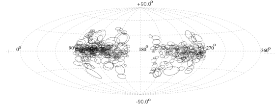
Fig. 1. Hammer-Aitoff projection of the GSc, centered on (l, b) = (180^\circ, 0^\circ)
