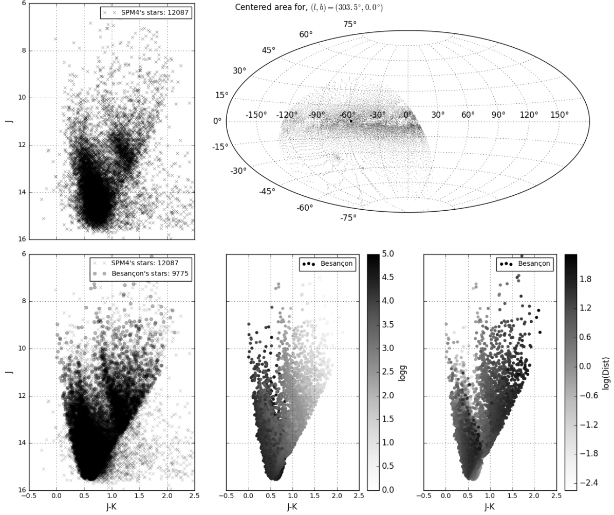
Fig. 1. J vs. J-K diagram of a field in the galactic disk
