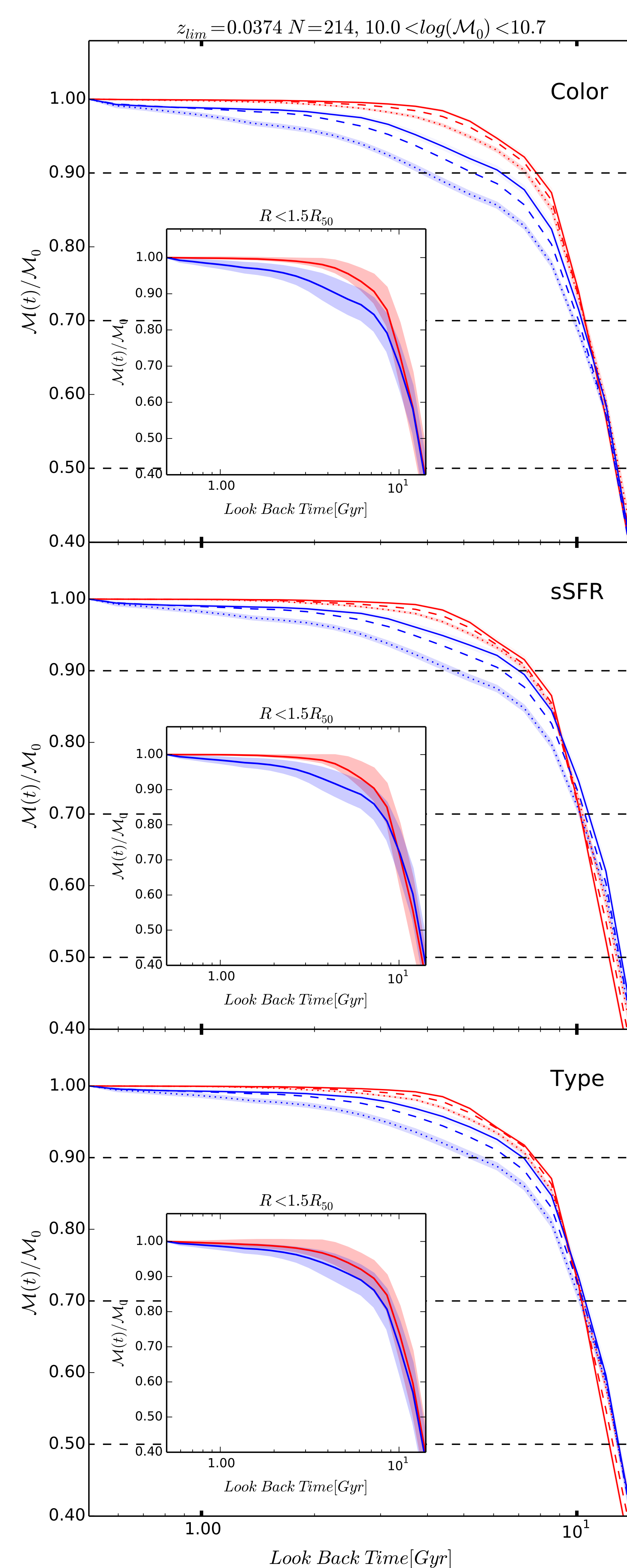
Dependence of the MGHs on galaxy properties
