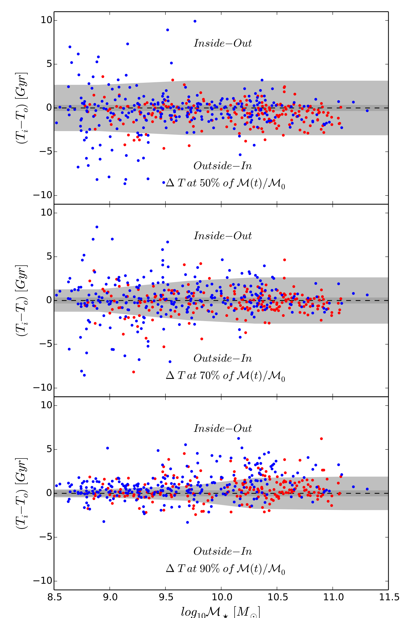
Individual mass assembly gradients
