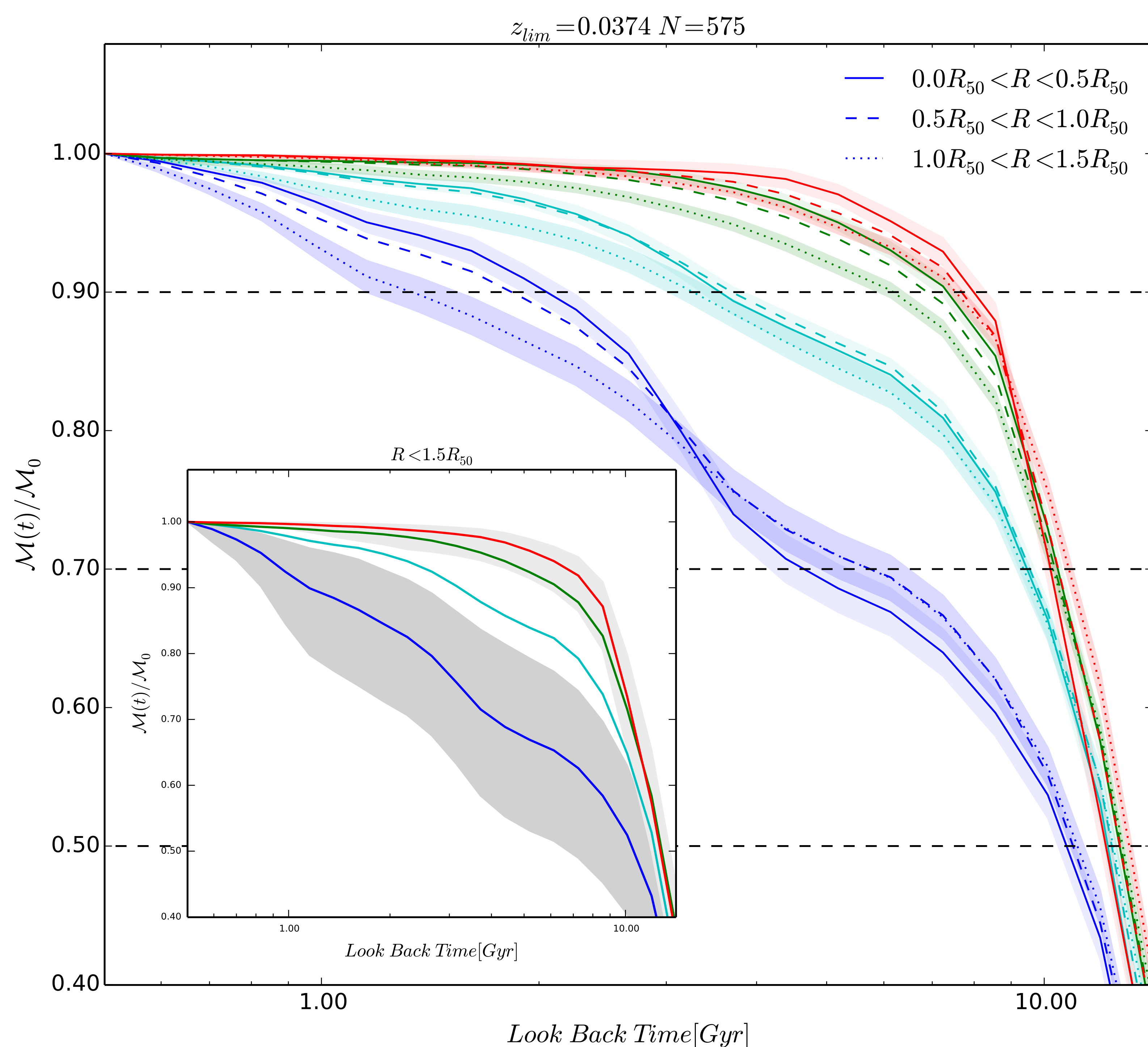
Mean MGHs in Stellar Mass Bins
