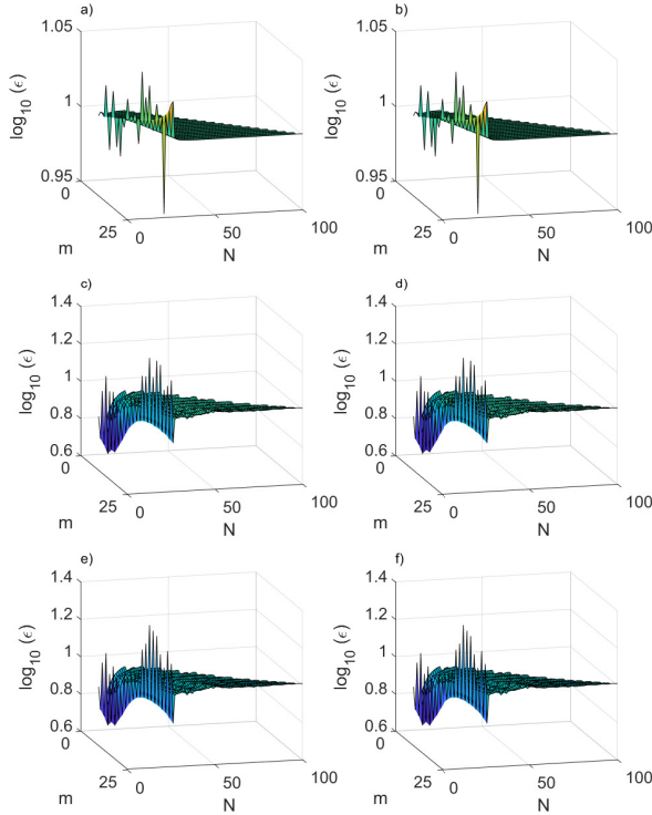
Figure 11. Ratio between errors of IVP in Inertial frame (a) and (b), BVP in Inertial frame (c) and (d), BVP in Rotating frame (e) and (f) and the reference IVP in Rotating frame in function of number of terms of polynomial series considered in the calculations. See Table 2 for caption details.
