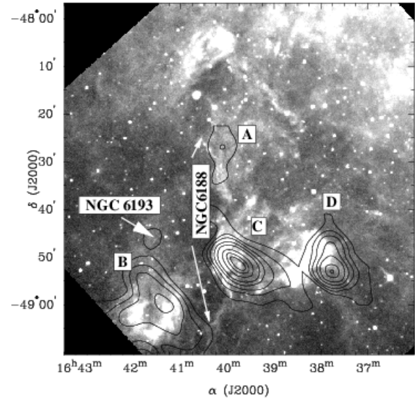
Fig. 1. Overlay of the MSX A-band emission (8 \mu m, grey-scale image) and the 13 CO emission (contour lines) associated with RCW 108. The objects referred to in the text are marked in this figure.
