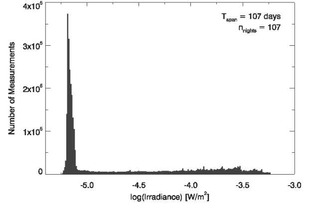
Fig. 4. Histogram of the measured irradiance during the night.
