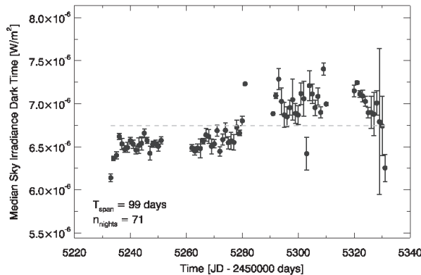
Fig. 3. Median night sky irradiance for Cerro Armazones.
