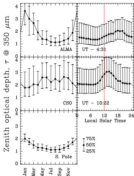
Fig. 5. Variations of the 350 \mu\text{m} zenith optical depth measured and on the Chajnantor plateau (ALMA), at the CSO on Mauna Kea, and at the South Pole. The error bars show the quartiles for each month or hour.
