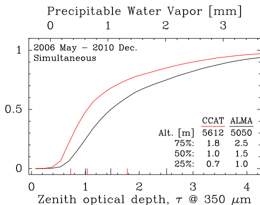
Fig. 6. Cumulative distributions of 350 \mu\text{m} zenith optical depth measured simultaneously near the summit of Cerro Chajnantor (CCAT) and on the Chajnantor plateau (ALMA). This PVW scale is only appropriate for the Chajnantor region.
